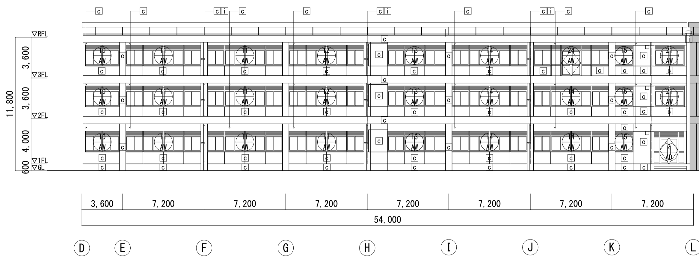
南立面図(4通り)S=1:200
