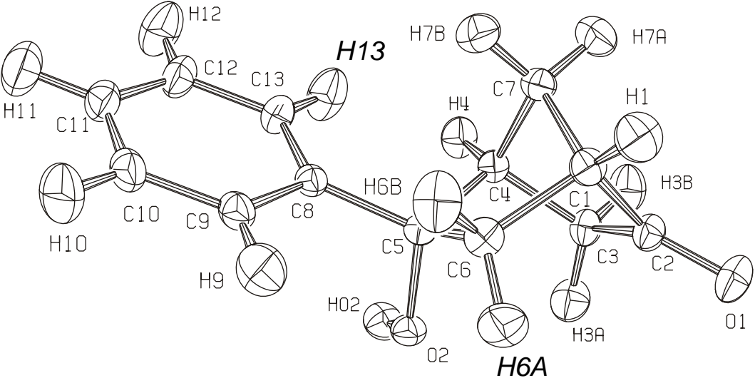
Phenyl-Hydroxyl-Norbornanone
